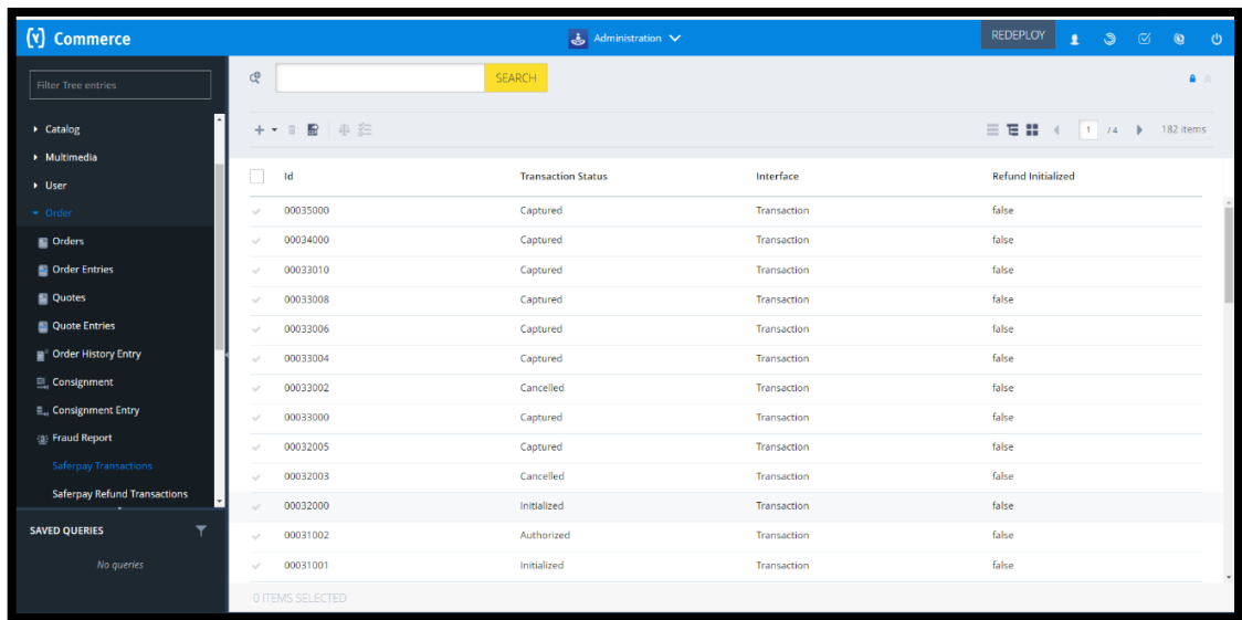
Figure 8: Transaction
