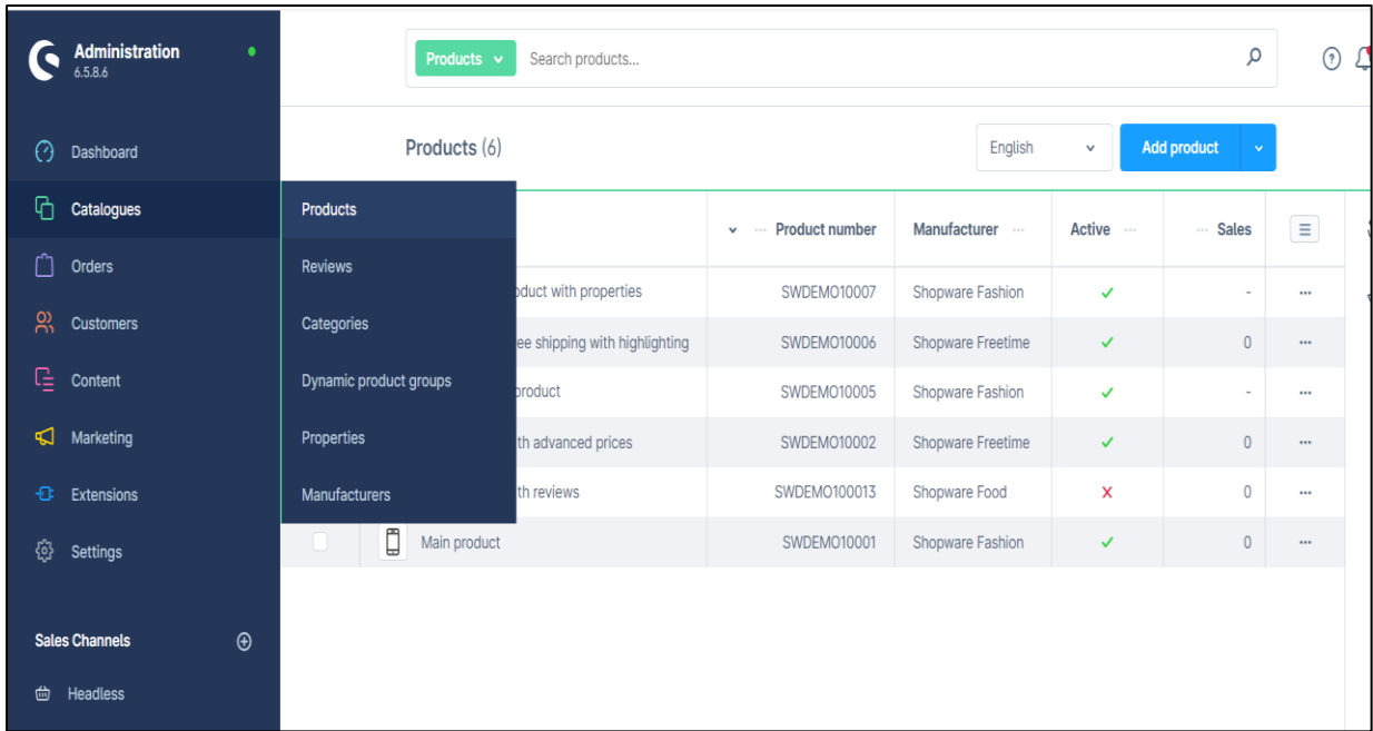
Figure 2. Products Tab
