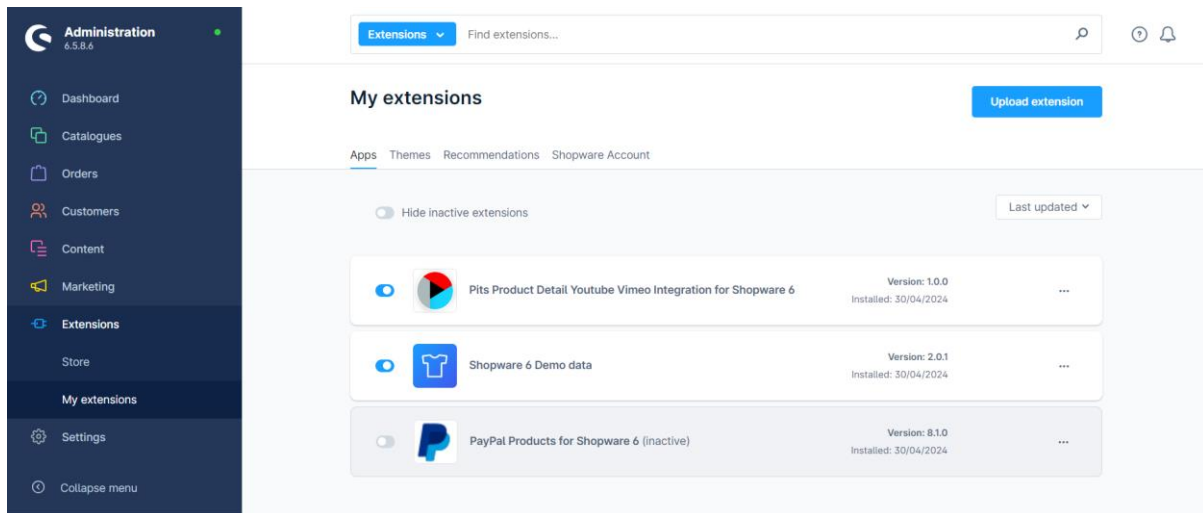
Figure 1. Module Configuration
